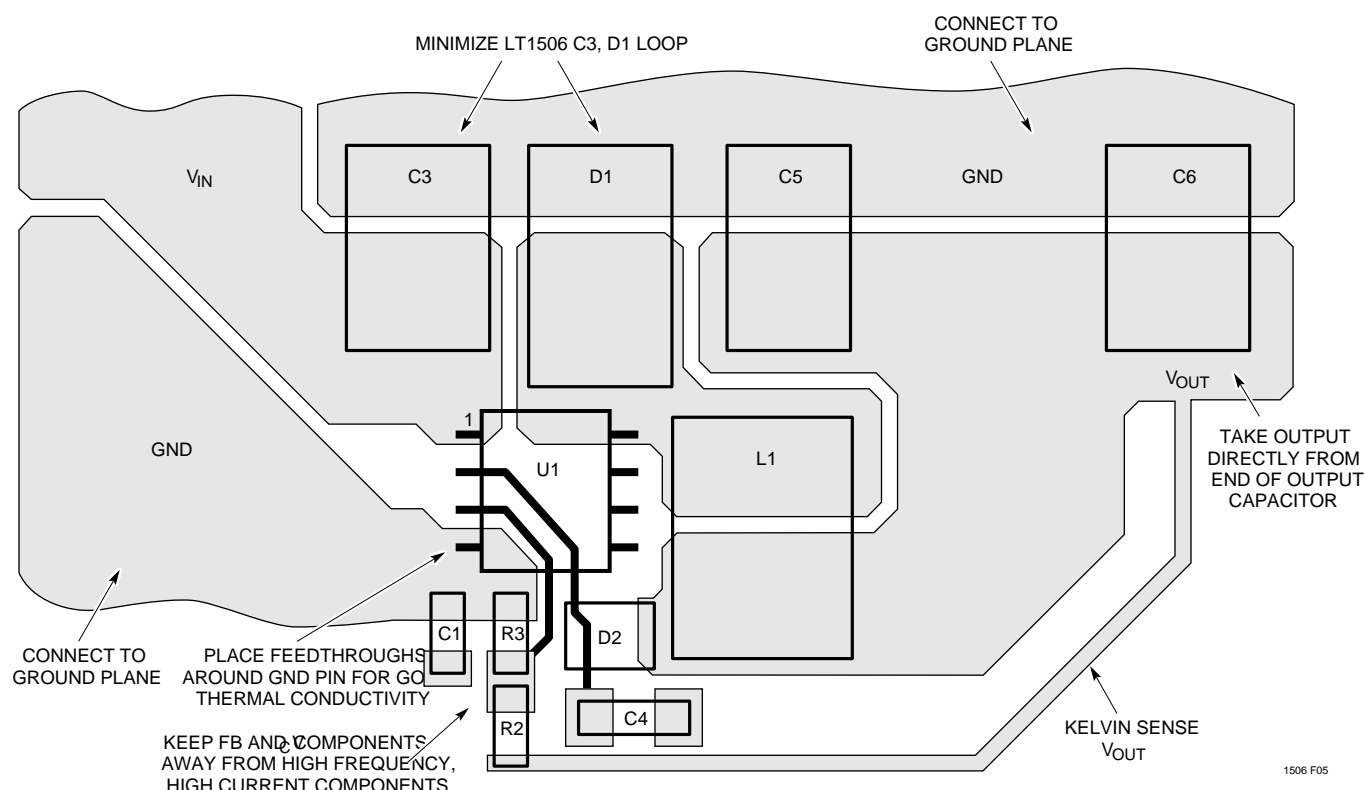
Figure 5. Suggested Layout (Topside Only Shown)
