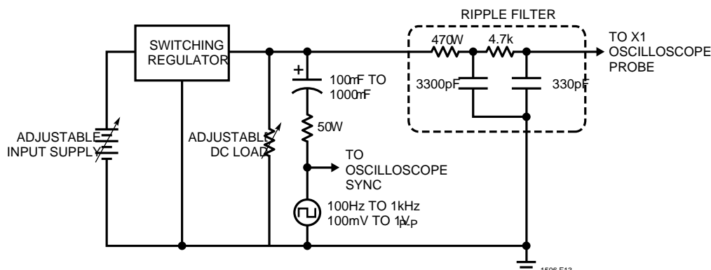
Figure 13. Loop Stability Test Circuit
