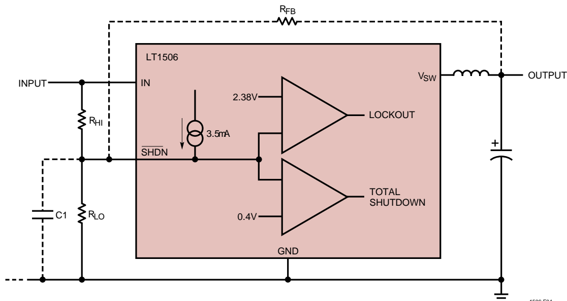
Figure 4. Undervoltage Lockout
