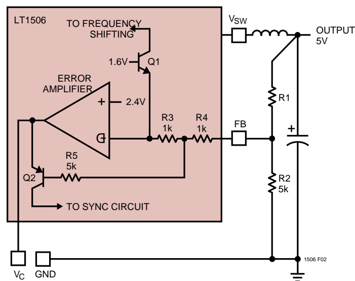
Figure 2. Frequency and Current Limit Foldback
