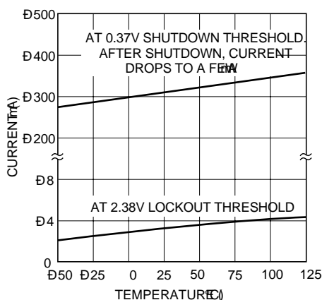
Shutdown Pin Bias Current
